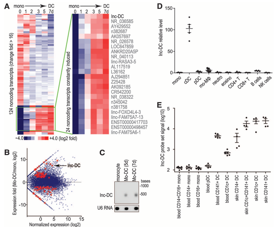
Fig. 1. lnc-DC is highly expressed in human DC subsets. (A) The cluster heat map shows lncRNAs with expression change fold >16 from microarray data ( P < 0.05 ). (B) Ratio of gene expression in Mo-DC to monocytes (vertical axis) and average expression of genes in Mo-DC versus that in monocytes (horizontal axis), presented as a Bland-Altman plot of our RNA-seq analysis. Highlighted in red are 99 lncRNAs with significant changes in expression (fold > 4, false discovery rate < 0.05). (C) Northern blotting of lnc-DC in monocytes and Mo-DC. U6 RNA serves as a loading control. Unless noted otherwise, all results in this and other figures were representative of at least three independent experiments. (D) qPCR detection of lnc-DC in immune cell subsets sorted from human peripheral blood. Data are normalized to glyceraldehyde-3-phosphate dehydrogenase (GAPDH) expression and monocytes (mono), which are set to a value of 1. NK cells, natural killer cells. (E) lnc-DC expression levels (signal intensity of probe set ILMN_3200140) in distinct DC/mono subsets of human blood and skin from GSE35457 data.
